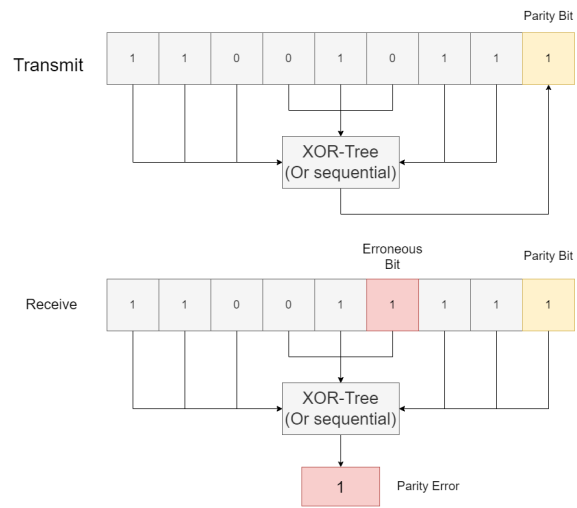
Figure 7: The parity bit is produced on the transmit side.
