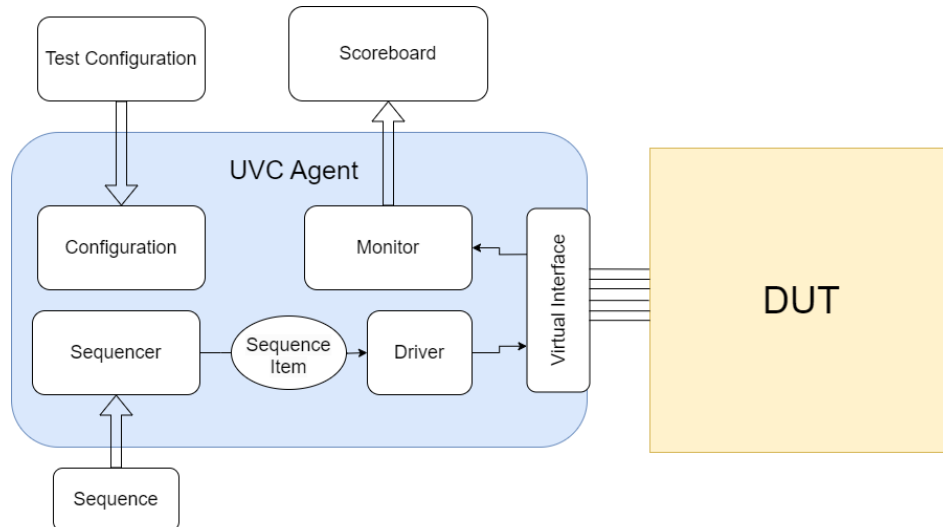
Figure 1: 10,000-foot view of how everything is interconnected within a UVM agent.
